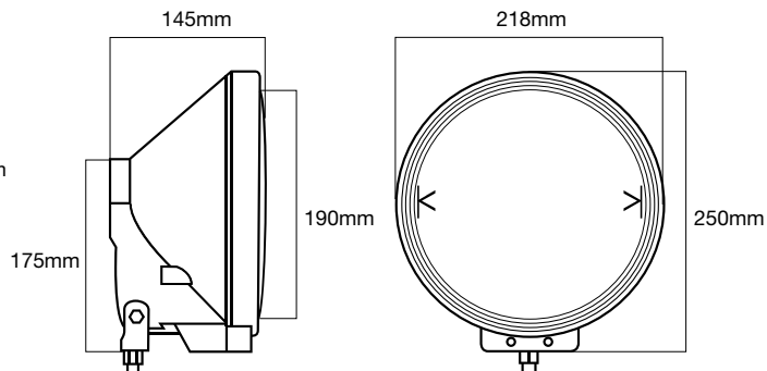
IVEGA220 and IHID001
