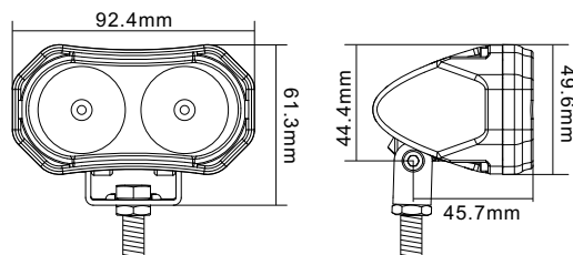
ILEDWL10 - (10/80Vdc Operating Voltage)
