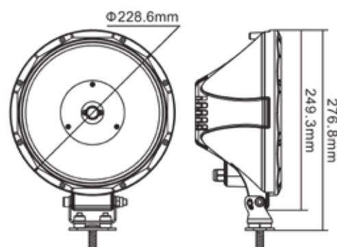
ILED9C - (12/24Vdc Operating Voltage)
