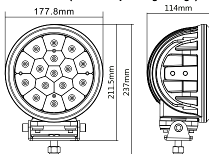
ILED7COMBO - (9/30Vdc Operating Voltage)
