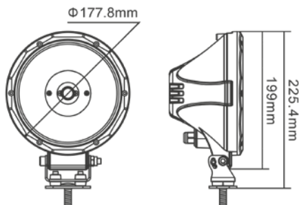
ILED7C - (12/24Vdc Operating Voltage)
