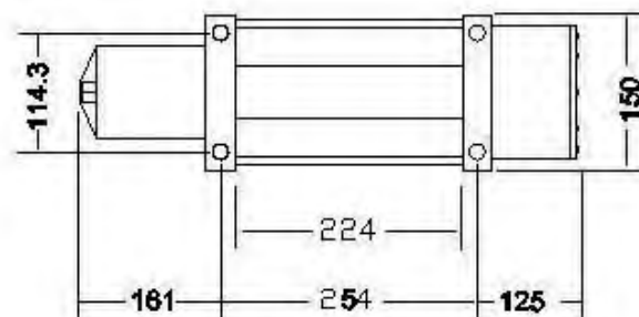
BOLTING PATTERN
